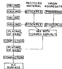
Figure 4. Construction process.
