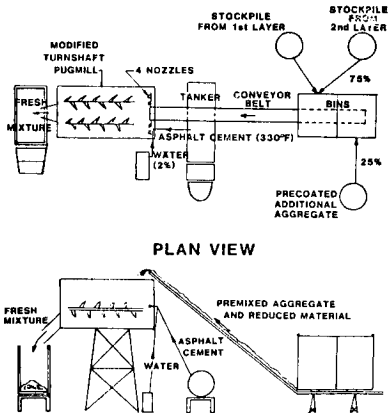
Figure 5. Mixing process.
