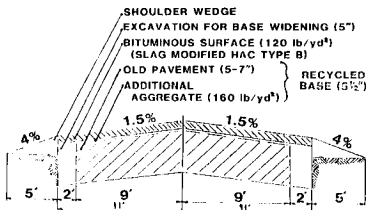
Figure 2. Pavement cross section.
