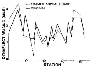
Figure 11. Maximum Dynaflect deflections 12 days after construction.
