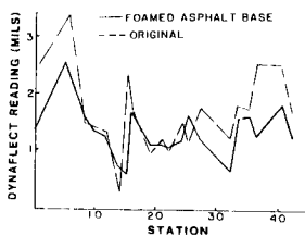
Figure 12. Maximum Dynaflect deflections 250 days after construction.
