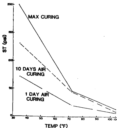
Figure 10. Effect of curing time on tensile strength.
