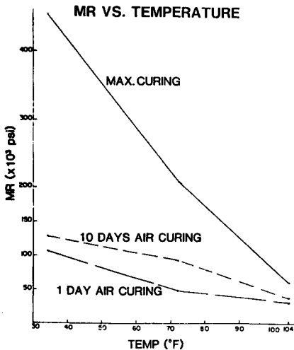
Figure 9. Effect of curing time on resilient modulus.
