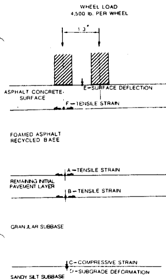
Figure 2. Typical pavement cross section used in analysis.
