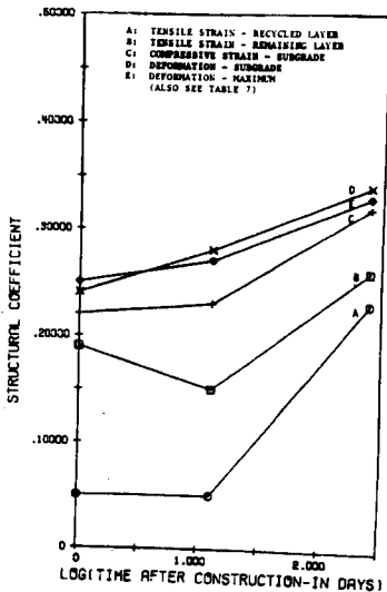
Figure 5. Effect of time after construction on structural coefficients: strains and deformations.
