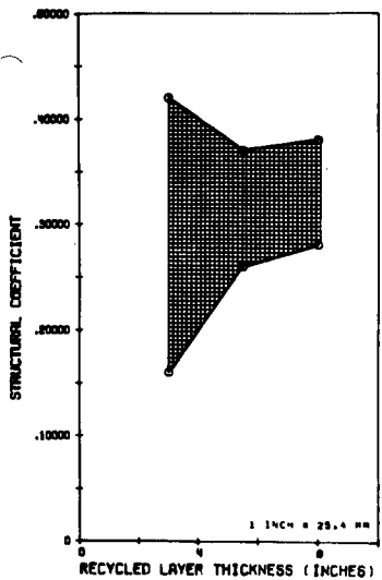
Figure 9. Recommended ranges of structural coefficients.
