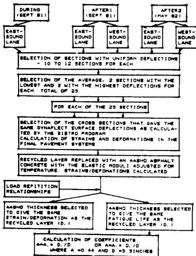
Figure 1. Procedure for determination of structural coefficients.
