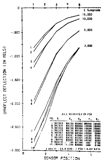
Figure 3. Influence of layer moduli on deflection basin.
