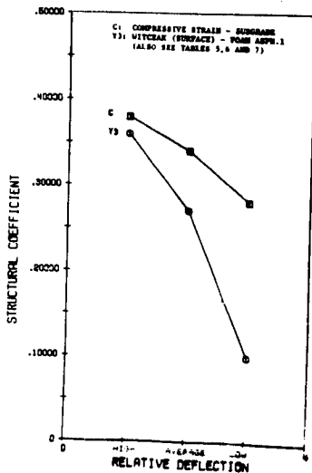
Figure 6. Coefficients based on controlling criteria.
