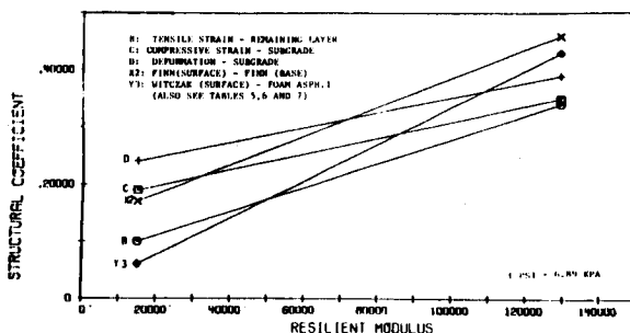
Figure 8. Relations between resilient modulus and structural coefficient.
