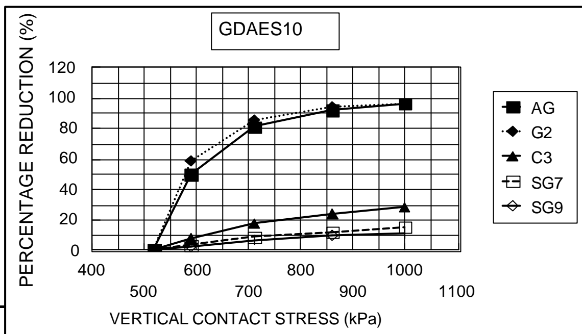
Figure 3: Percentage Reduction in Calculated Layer Life As A Result of Increased Contact Stress on Pavement GDAES10 (GDAES10: Granular Base, Dry, Category A, Traffic Class: ES10 (TRH 4, 1996) The layer codes AG; G2; C3; SG7; SG9 are from TRH 4 (1996)).
